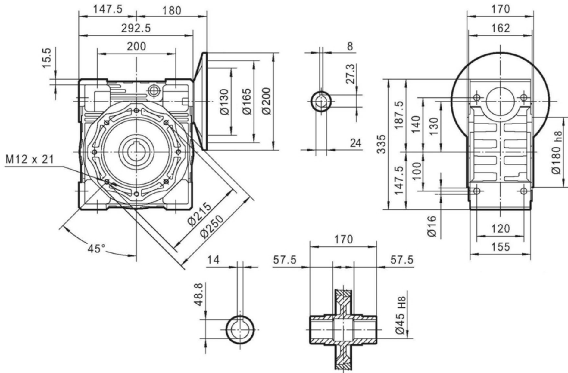
PMRV 130 90B5
