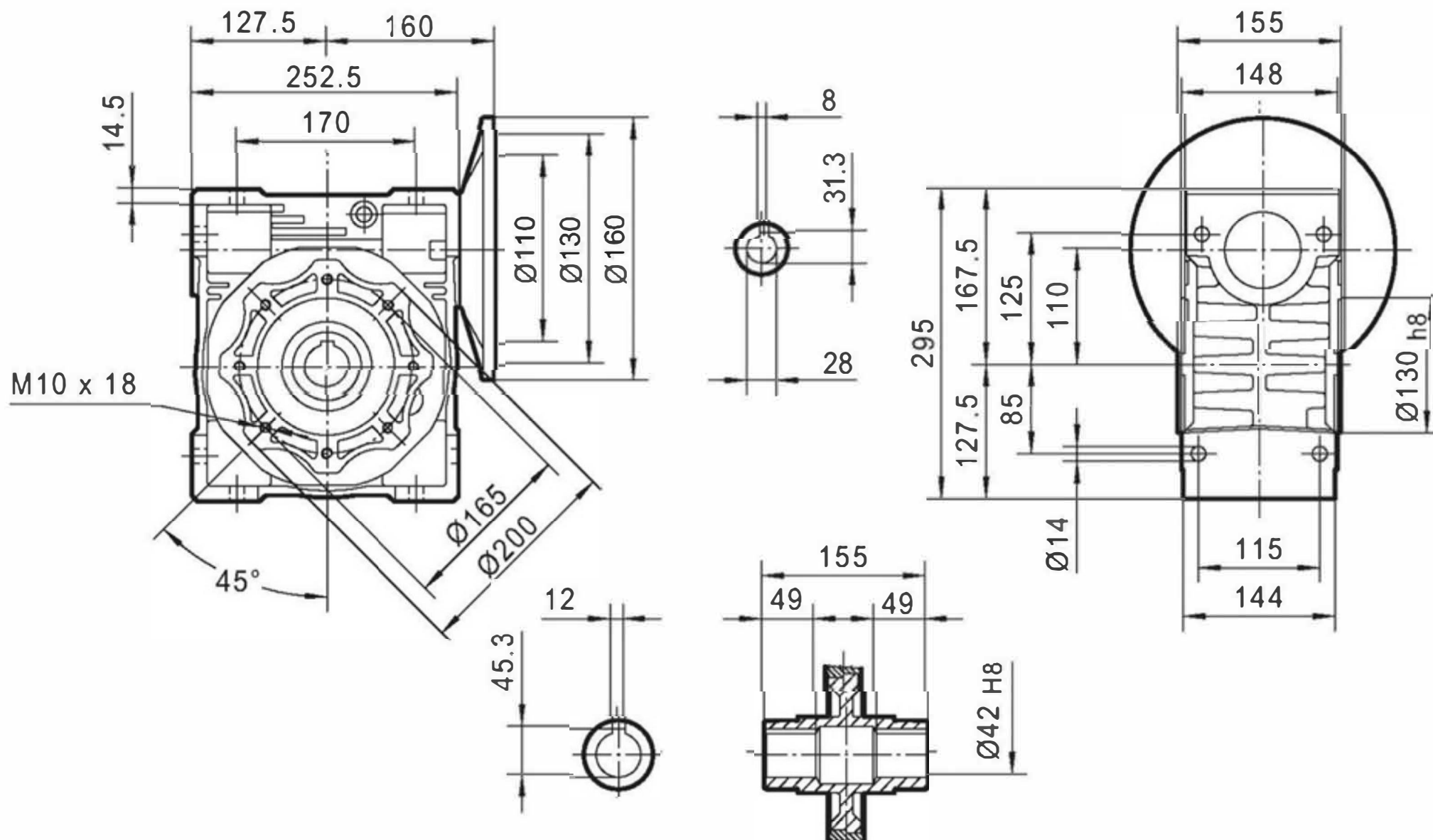
NMRV 110 100/112B14
